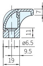
ESP-010-□ 皿頭內六角螺絲
